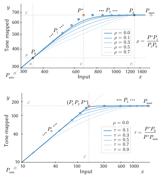
Figure 4: Tone mapping operator formulated by cubic Bézier curve.
